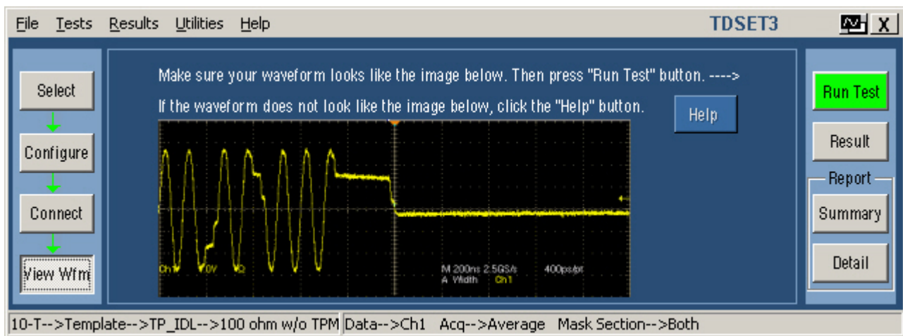
Figure 13-4: 10BASE-T View Waveform for TP_IDL without TPM
