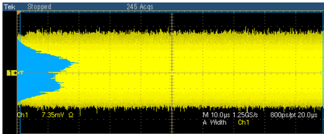
Figure 10-25: Waveform for 10BASE-T Common mode Voltage
