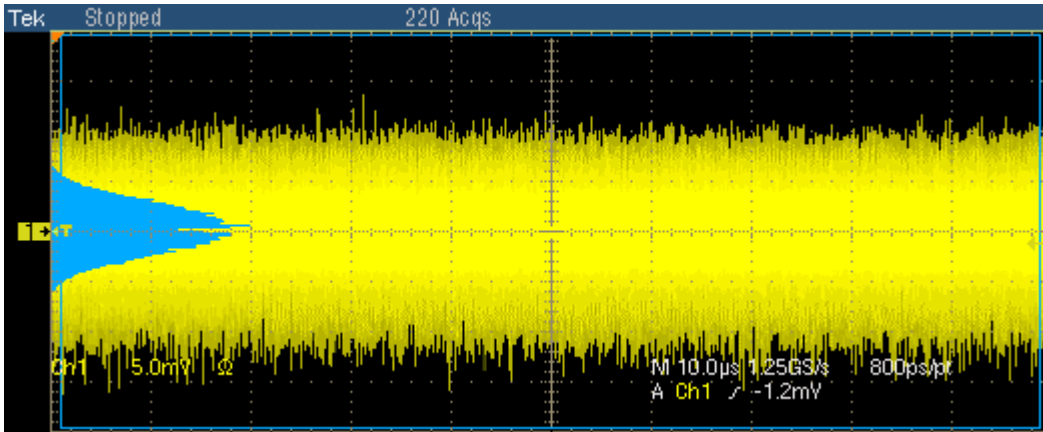
Figure 8-24: Waveform for 1000BASE-T Common mode Voltage
