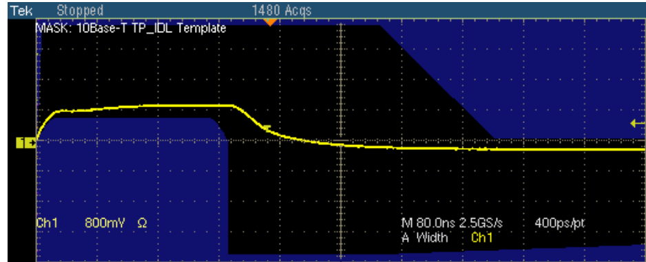
Figure 10-11: Waveform for 10BASE-T TP_IDL Head
